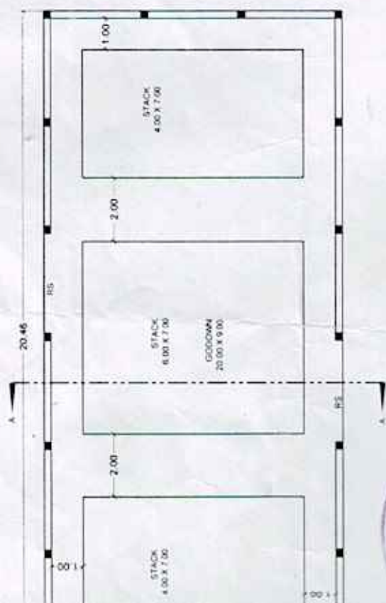
PROPOSED G.F. PLAN SCALE: 1/100
